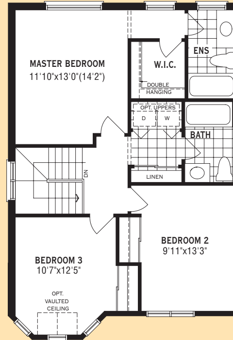
Second Floor Plan 3 Bedroom
