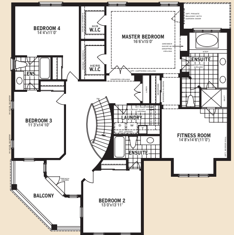
Opt. Second Floor Plan 4 Bedrooms And 3 Baths With California Master
