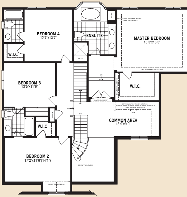
Opt. Second Floor Plan With 4 Bedrooms And 3 Baths With Common Area (Only Available With Optional Ground Floor Plan) (3796 Sq. Ft. Including 152 Sq. Ft. O.T.B.)
